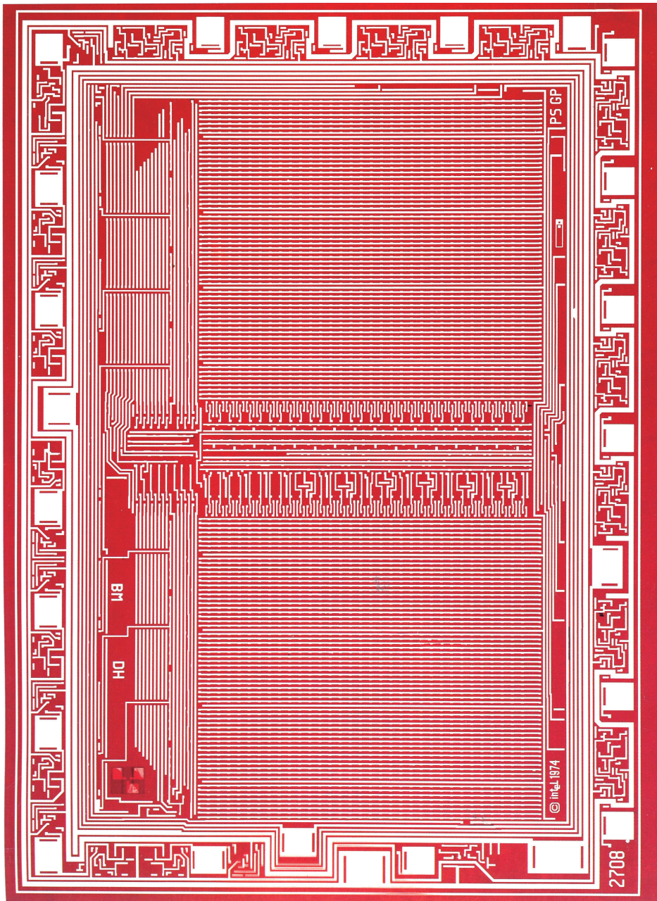
Intel Corporation, 1974. Erasable Programmable Read-Only Memory Chip (EPROM).
